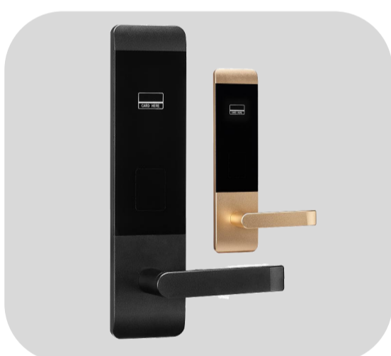
Model: X5 Colors: gold , black Material: Aluminium alloy Size: 300*75*12mm
