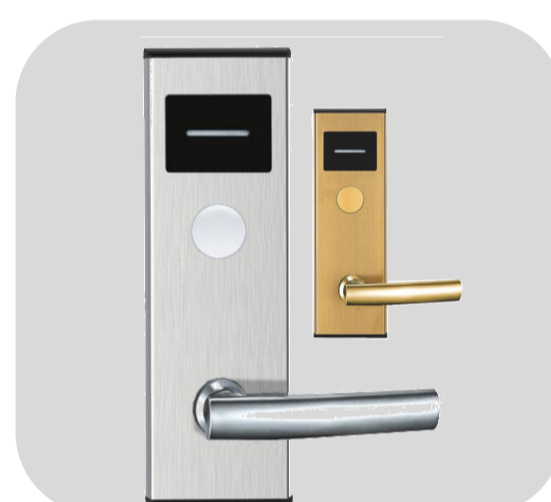
Model: B001 Colors: gold , silver Material: Stainless steel Size: 247*76*20mm
